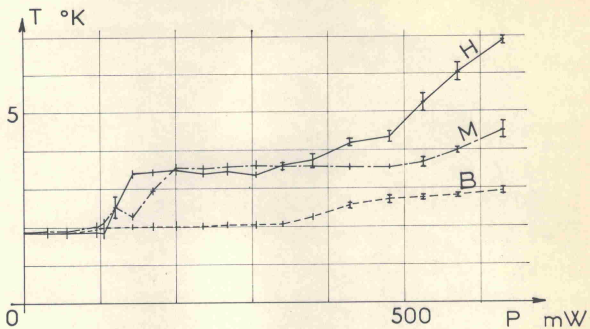
FIG. 5 : Superfluid helium T = 1.85 K; P = 335 mm Hg
