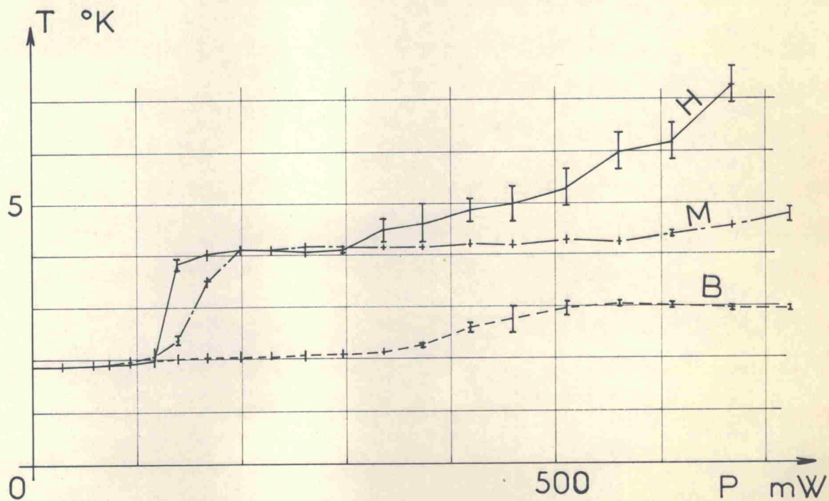
FIG.6 : Superfluid helium T = 1.85 K ; p = 1 atm
